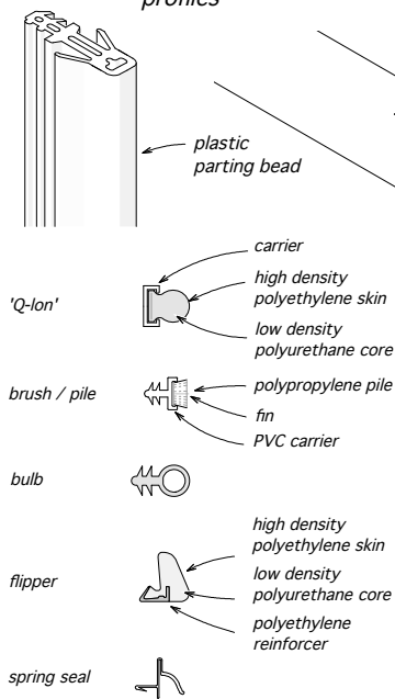
Typical draught seal profiles
