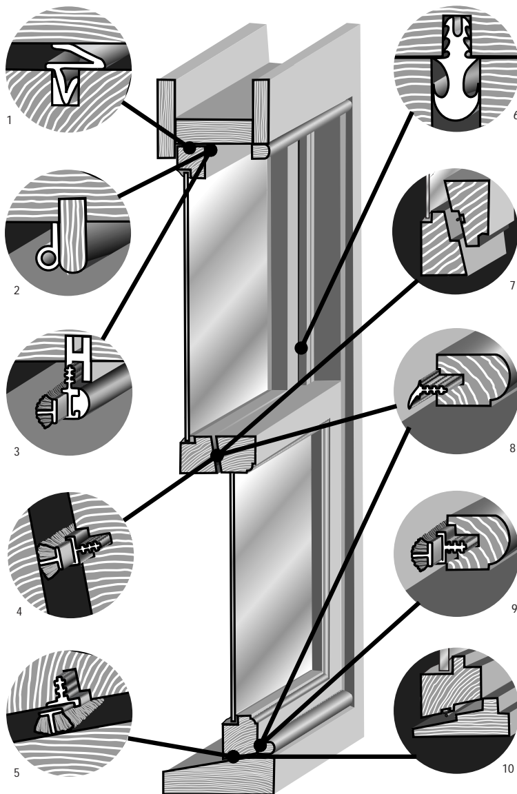
Figure 7 1 Plastic or sprung metal 'V' or 'Z' strip 2 Glued or pinned silicone rubber tubing 3 Parting bead (Ventrolla) 4 Meeting rail brush (Ventrolla) 5 Bottom sash/sill brush (Ventrolla) 6 Parting bead weatherstrip (Mighton) 7 Brush for meeting rails (Draftseal) 8 Standard weatherstrip (Mighton) 9 Staff bead or button rod (Ventrolla) 10 Silicone seal (Draftseal) (Digital image by Robyn Pender from English Heritage original line drawing)
