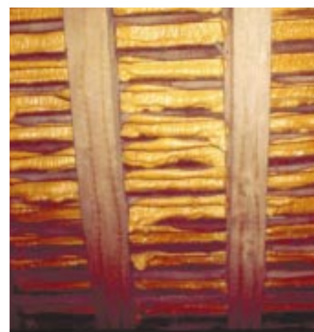
Figure 14 Sprayed foam used as a way of avoiding stripping a 'nailed' roof and providing some insulation is NOT recommended good practice on a historic building. (Photograph courtesy of Kevin Stubbs, Bursledon Brickworks Conservation Centre)
